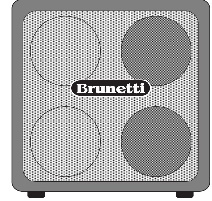
8Ω - 8Ω CABINET 4X12" USING ONLY 2 SPEAKERS
